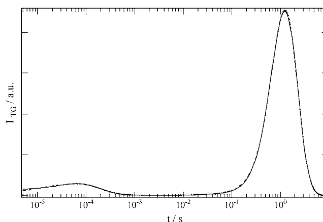
FIGURE 5 Observed TG signal (dotted line) after photoexcitation of intact phy in the Tris buffer at q^2 = 3.0 \times 10^{10} \text{ m}^{-2} . The best fitted line with Eq. 4 is shown by the solid line.
